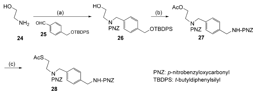
Scheme 4. Synthesis of 28 . Reagents: (a) (i) 25 , Na(OAc) 3 BH, AcOH, THF, rt; (ii) PNZ-Cl, NaOH, 1,4-dioxane, H 2 O; (b) (i) Ac 2 O, pyridine, DMAP, THF, rt; (ii) tetra- n -butylammonium fluoride, THF, rt; (iii) MsCl, i -Pr 2 NEt, THF, 0 °C; (iv) NaN 3 , DMF, rt; (v) PPh 3 , H 2 O, THF, rt; (vi) PNZ-Cl, NaOH, 1,4-dioxane, H 2 O; (c) (i) NaOH, MeOH, rt; (ii) PPh 3 , DIAD, thioacetic acid, THF, 0 °C.
