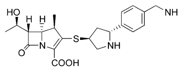
Figure 1. Chemical structure of 1a .
