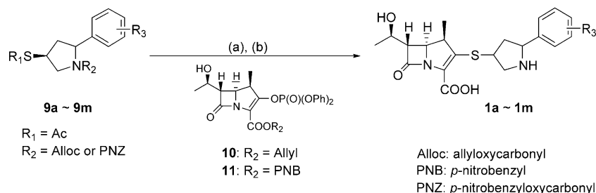
Scheme 2. Synthesis of 1a–1m . Reagents: (a) (for 1a , 1b , 1c , 1d , 1e , 1f , 1g , 1h , 1i , 1j , 1k and 1m ) (i) \text{NaOH} , MeOH, 0^\circ\text{C} ; (ii) 10 , i\text{-Pr}_2\text{NEt} , \text{CH}_3\text{CN} ; (iii) (\text{PPh}_3)_2\text{PdCl}_2 , n\text{-Bu}_3\text{SnH} , \text{H}_2\text{O} , \text{CH}_2\text{Cl}_2 , 0^\circ\text{C} ; (b) (for 1l ) (i) \text{NaOH} , MeOH, 0^\circ\text{C} ; (ii) 11 , i\text{-Pr}_2\text{NEt} , \text{CH}_3\text{CN} ; (iii) \text{H}_2 , \text{Pd/C} , rt.
