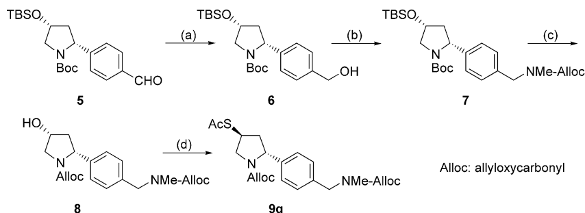
Scheme 1. Synthesis of 9g . Reagents: (a) \text{NaBH}_4 , MeOH, 0^\circ\text{C} ; (b) (i) \text{MsCl} , \text{Et}_3\text{N} , \text{CH}_2\text{Cl}_2 , -30^\circ\text{C} ; (ii) \text{MeNH}_2/\text{MeOH} , rt; (iii) \text{Alloc-Cl} , 0^\circ\text{C} ; (c) (i) \text{HCl-MeOH} , reflux; (ii) \text{Alloc-Cl} , 0^\circ\text{C} ; (d) (i) \text{MsCl} , \text{Et}_3\text{N} , \text{CH}_2\text{Cl}_2 , -40^\circ\text{C} ; (ii) \text{AcSK} , DMF, 60^\circ\text{C} .
